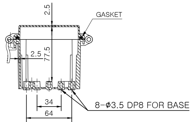
SECTION B-B
